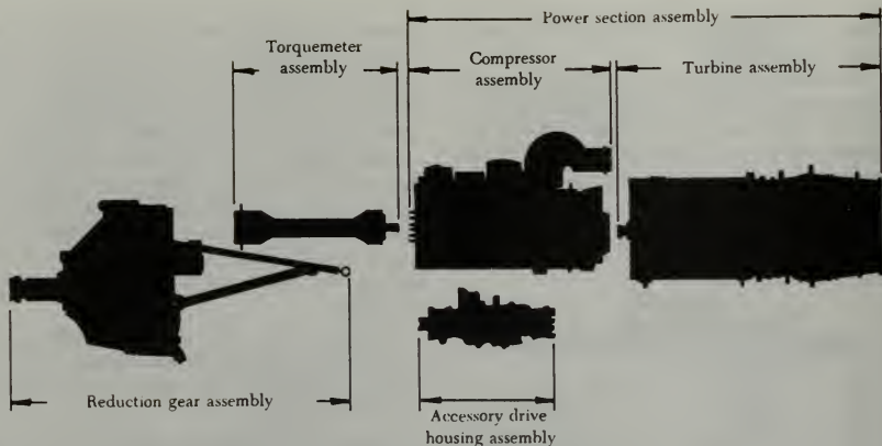
FIGURE 1-68. Turboprop engine major components.
